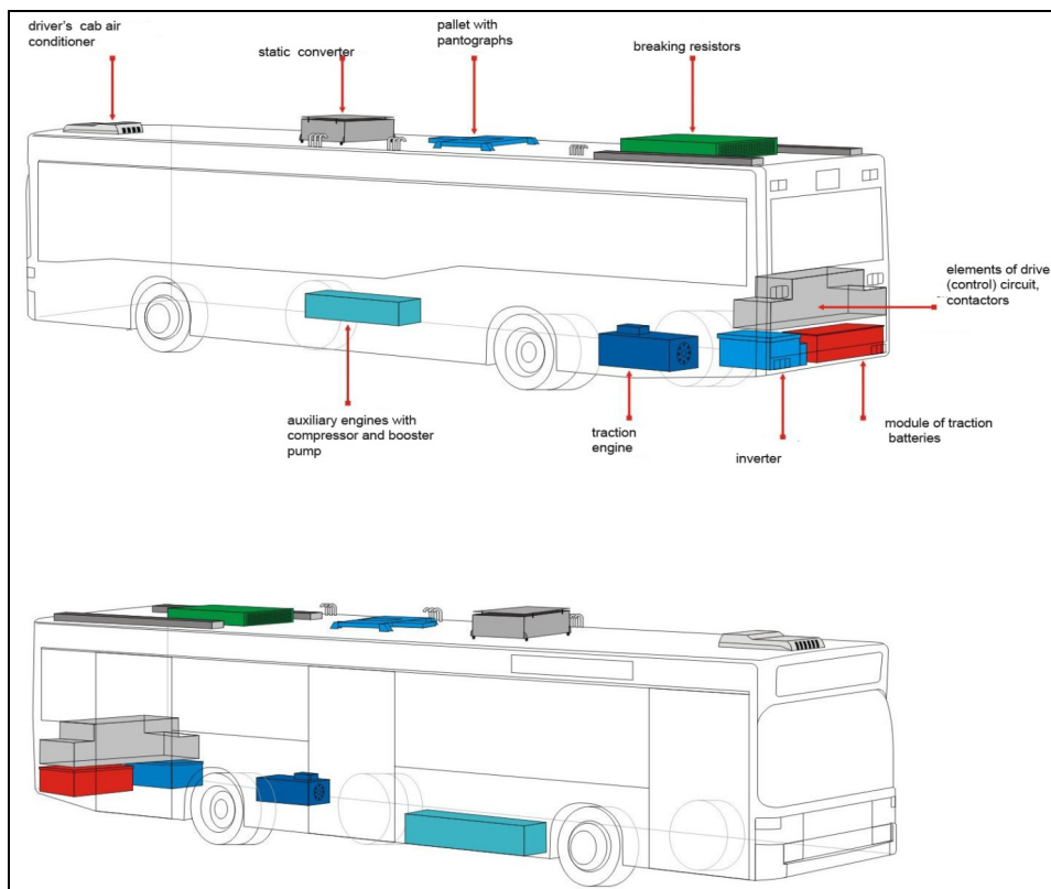
Fig. 12. Machinery arrangement in trolleybus O405N equipped with impulse (chopper) drive (Authors: Maciej Beister, Marcin Połom)
