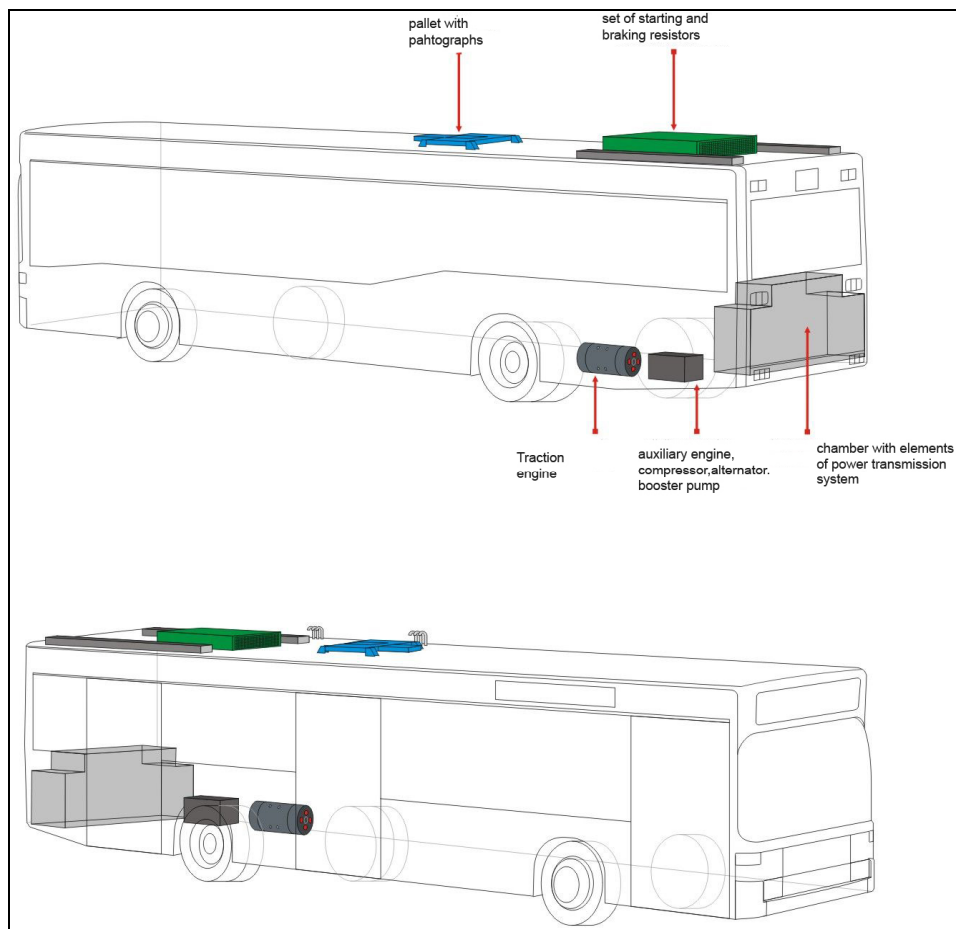
Fig. 6. Machinery arrangement in trolleybus O405N equipped with contactor drive (Authors: Maciej Beister, Marcin Połom)
