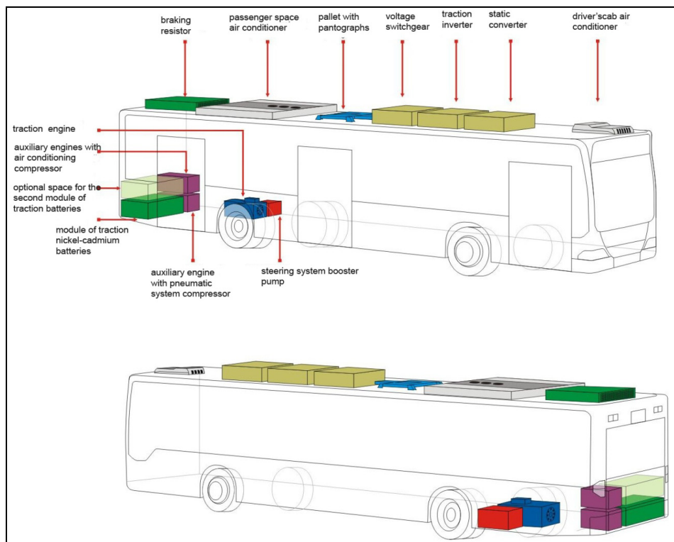
Fig. 17. Machinery arrangement in trolleybus O530 equipped with asynchronous drive (Gdynia) (Authors: Maciej Beister, Marcin Połom)
