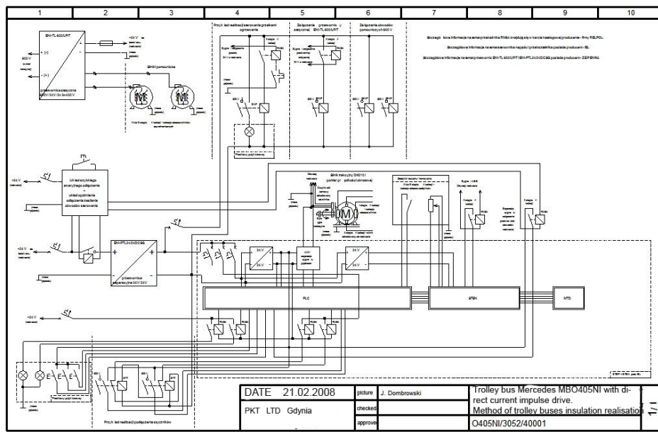
Fig. 19. Scheme of method of trolleybuses insulation realisation
