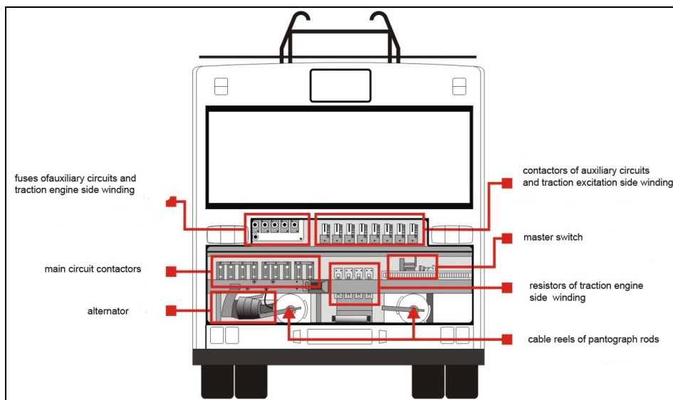
Fig. 7. Electrical drive machinery arrangement in combustion engine compartment of trolleybus O405N equipped with contactor drive (Authors: Maciej Beister, Marcin Polom)
