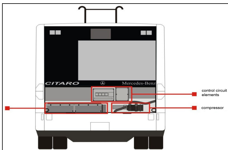
Fig. 16. Electrical drive machinery arrangement in combustion engine compartment of O530 trolleybus equipped with asynchronous drive (Szeged) (Authors: Maciej Beister, Marcin Polom)
