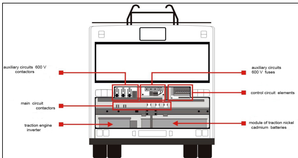
Fig. 13. Electrical drive machinery arrangement in combustion engine compartment of O405N trolleybus equipped with impulse (chopper) drive (Authors: Maciej Beister, Marcin Połom)
