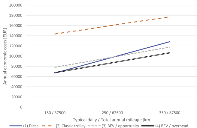
Fig. 4. Annual economic costs of operation of a line (including externalities) under technology variants – assuming real Polish energy-mix. Source: own work based on the (ELIPTIC Project, 2018; TROLLEY 2.0, 2020).
